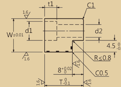
3處安裝螺栓孔 Mounting bolt hole:3
