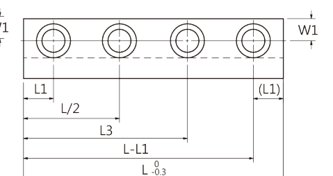
4處安裝螺栓孔 Mounting bolt hole:4
